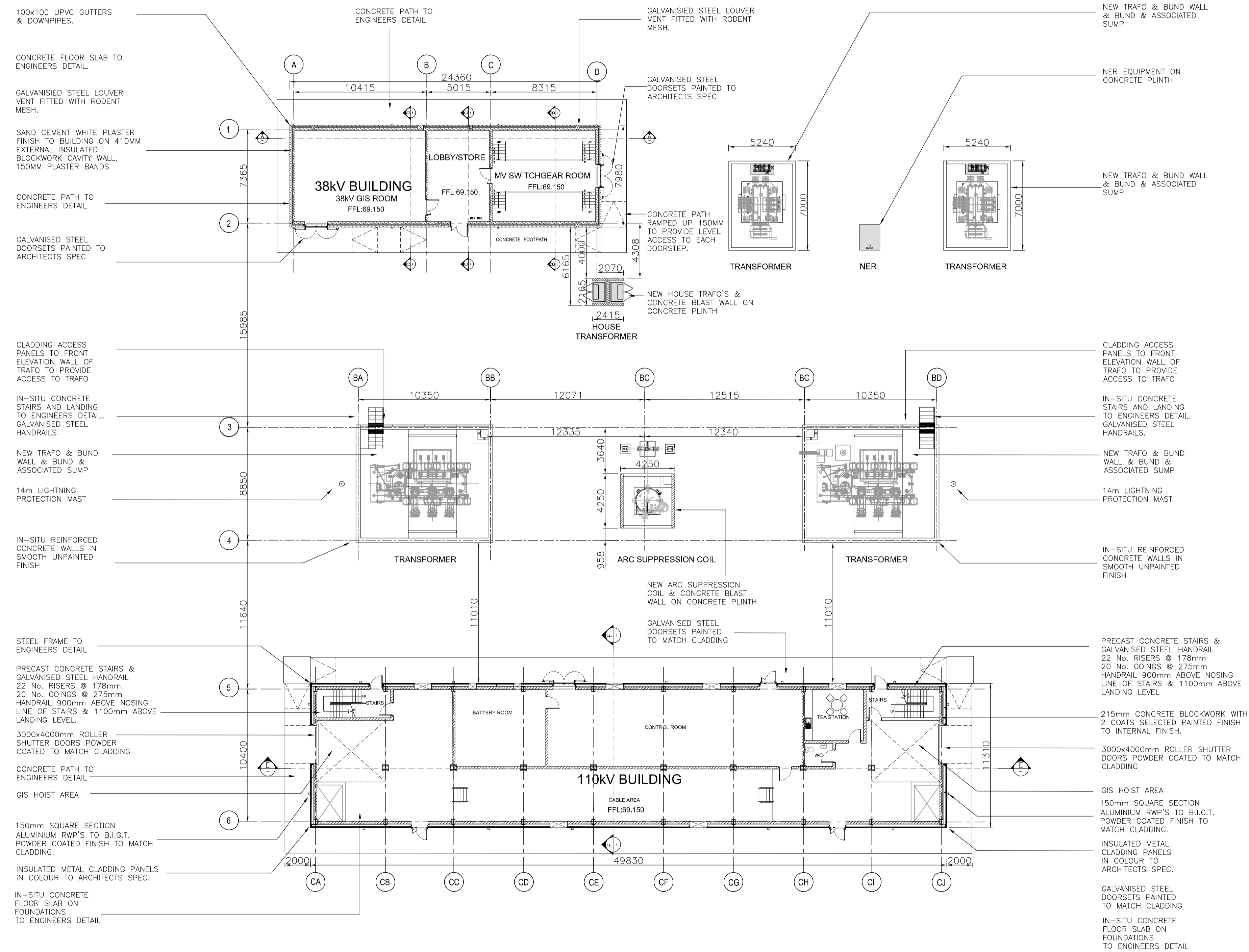
GROUND FLOOR PLANS SCALE 1:200
